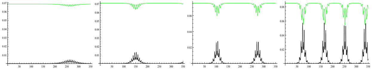
Figure 5: The energies \mathcal{E}^\theta(t) (black) and \mathcal{E}^y(t) (green) in (12). From left to right, the values of y_0 are: y_0 = 0.335 , y_0 = 0.34 , y_0 = 0.35 , y_0 = 0.37 .
