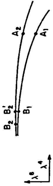
Fig. 1. Neighboring trajectories in the \lambda_1 - \lambda_6 plane.
