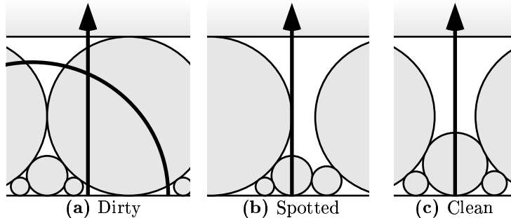
FIGURE 2. The various possibilities for a geodesic intersecting the cusp.
