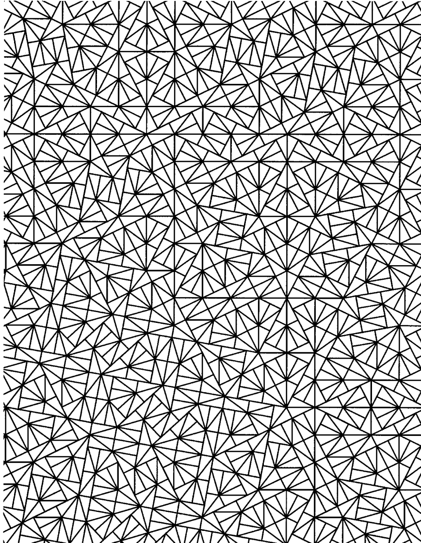
Figure 6. A pinwheel tiling.
