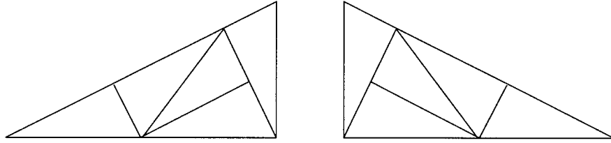
Figure 7. The substitution for pinwheel tilings.
