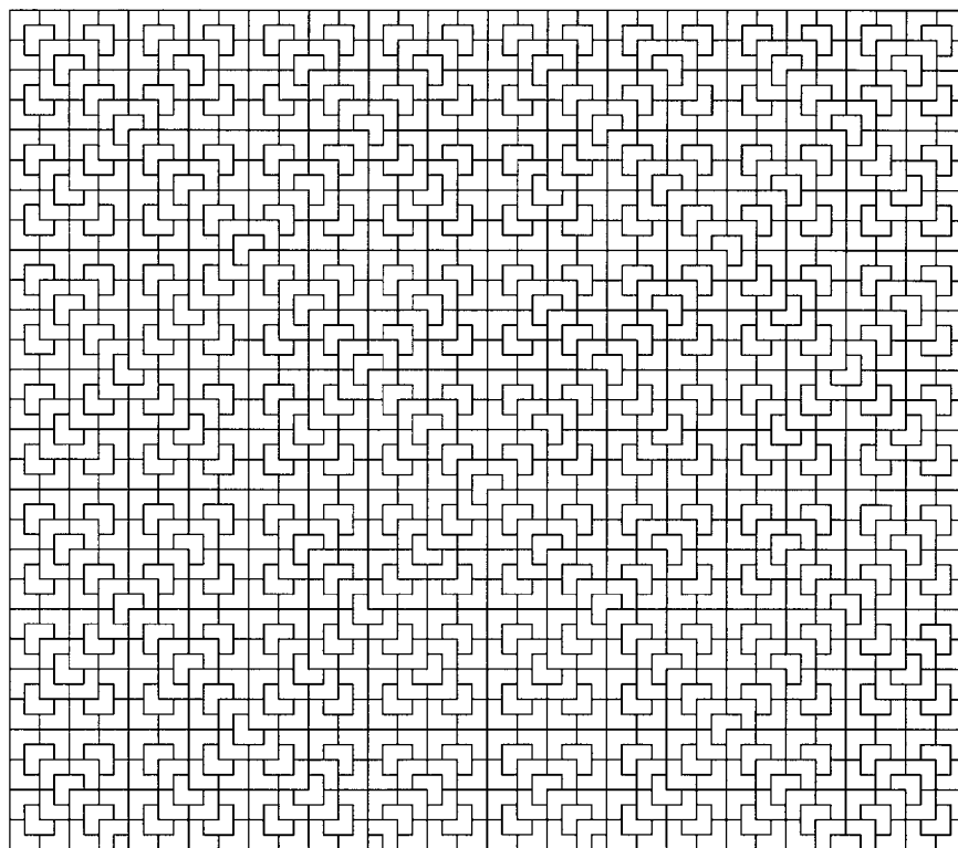
Figure 1. A chair tiling.
