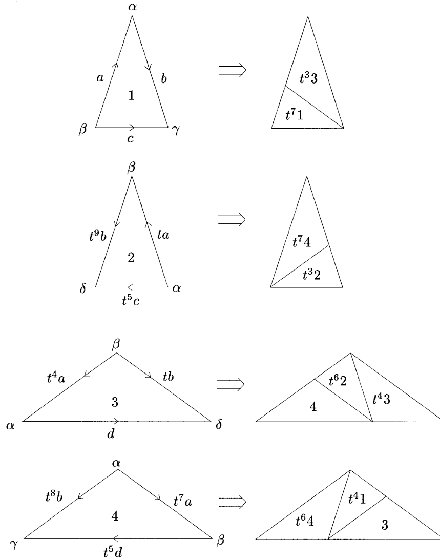
Figure 9. The Penrose substitution in detail.
