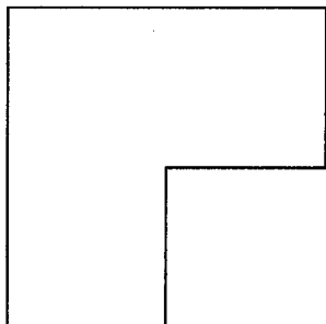
Figure 2. The chair tile.
