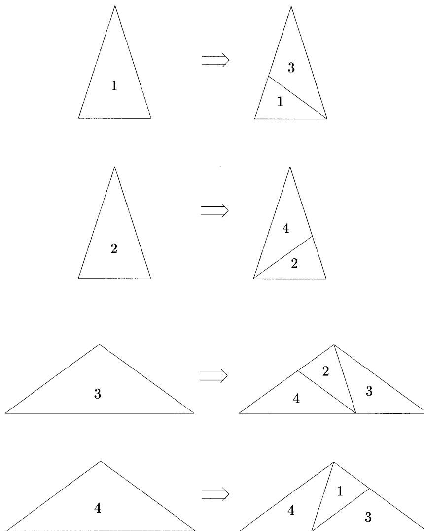
Figure 5. The Penrose substitution.
