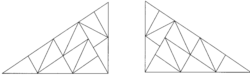
Figure 8. The substitution for (2,3) pinwheel tilings.
