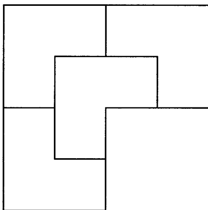
Figure 3. The chair substitution.
