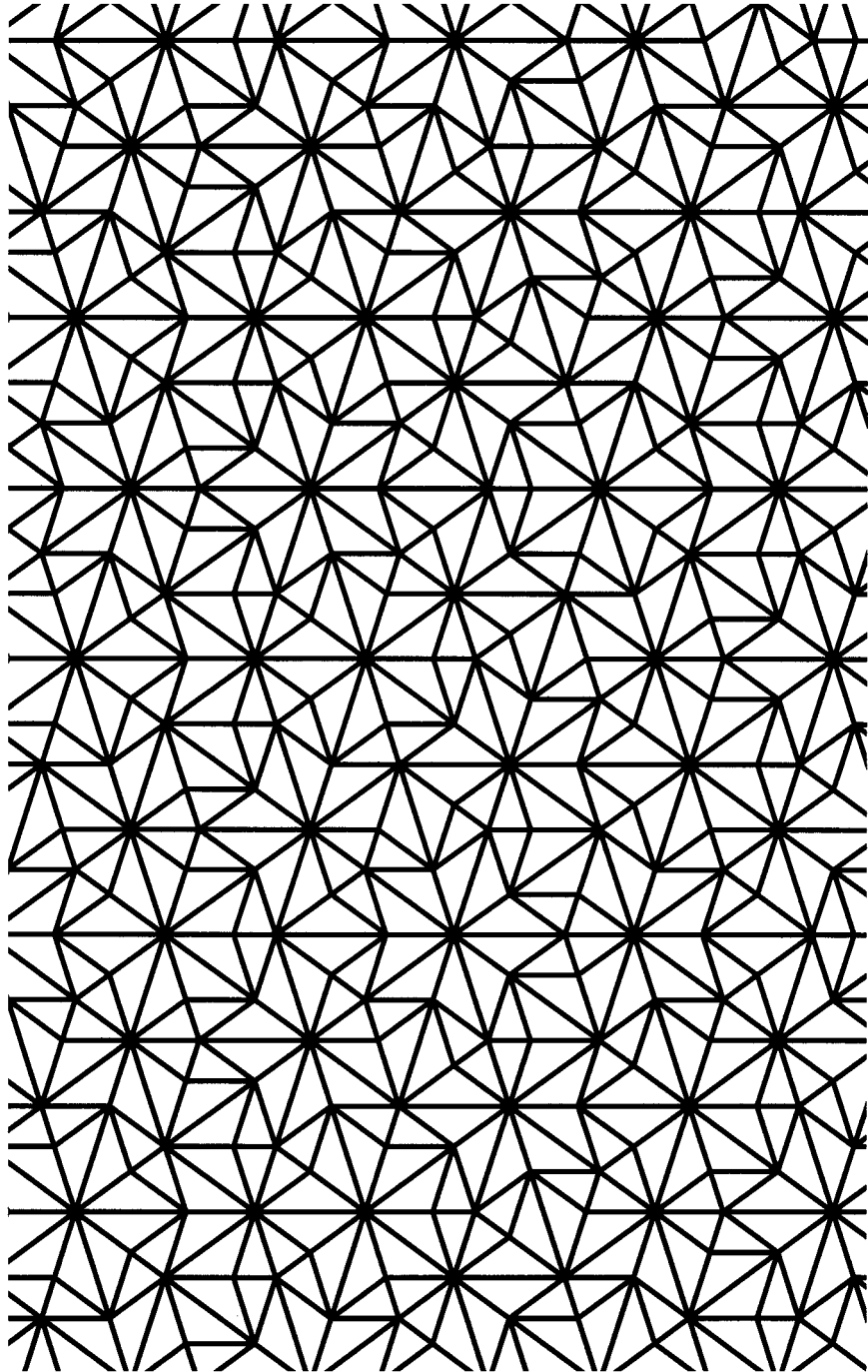
Figure 4. A Penrose tiling.
