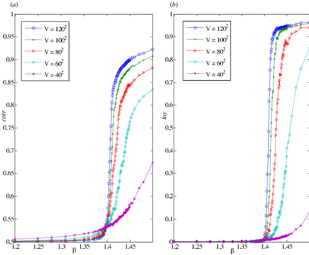
Figure 5. (a) The graph of corr versus \beta at \mu = 0.15 , for volumes V = 40^2 to V = 120^2 . (b) The graph of lay versus \beta at \mu = 0.15 , for volumes V = 40^2 to V = 120^2 .
