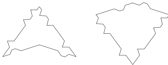
Figure 1. The kite and dart tiles
