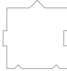
Figure 3. The hyperbolic Penrose tile
